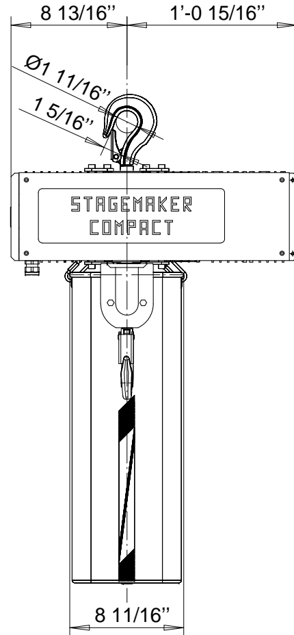
SECOND BRAKE OPTION
